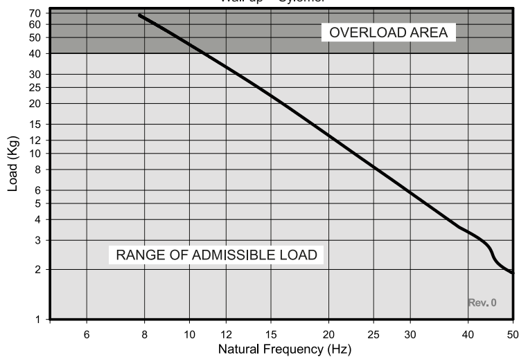
NATURAL FREQUENCY GRAPH
