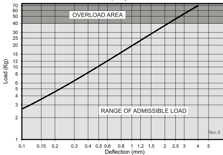
LOAD-DEFLECTION GRAPH
